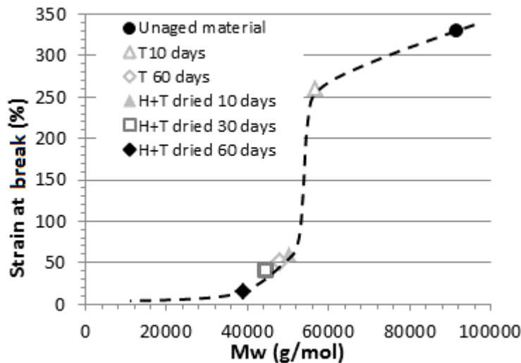
36 37 38 39 40 41 42 43 44 Figure 19 Strain at break as a function of weight average molar mass obtained after T ageing (110°C) and H+T ageing 45 (pH4/110°C). 46
