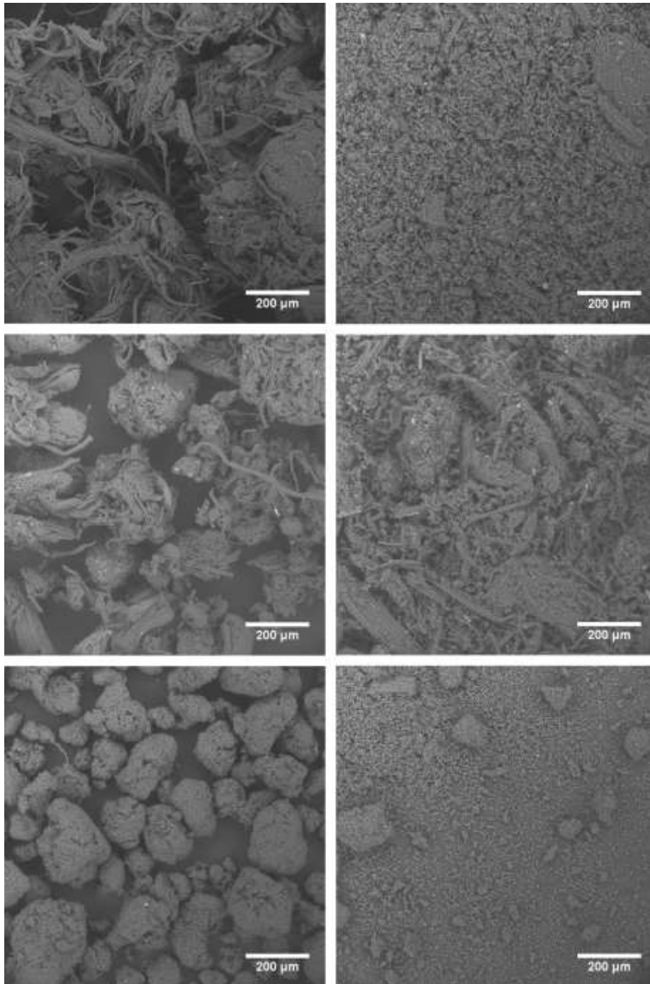
Figure S1. SEM images of steam-exploded samples (R0, left) {Auxenfans, 2017 #844} and of residual solids fraction R1 from hydrolysed R0 samples (right, this study) for wheat straw, miscanthus and poplar (from top).
