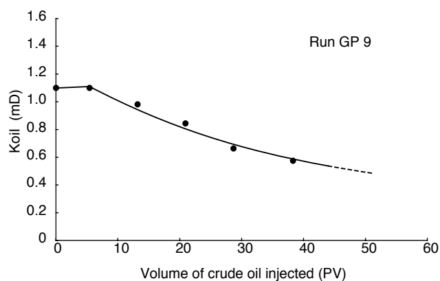
Figure 6 Oil permeability reduction in a tight Pflaz sandstone.
