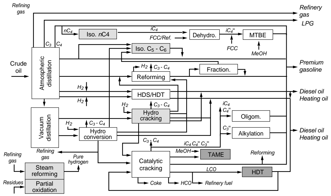
Figure 3 2010-2020 refining scheme.
