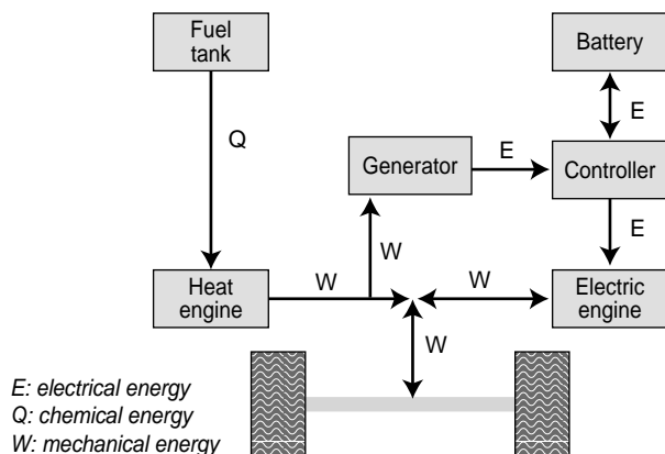
Figure 10 Combinations of heat and electric engines for hybrid vehicle.
