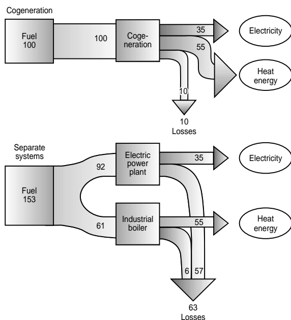
Figure 5 Energetic balance of cogeneration.
