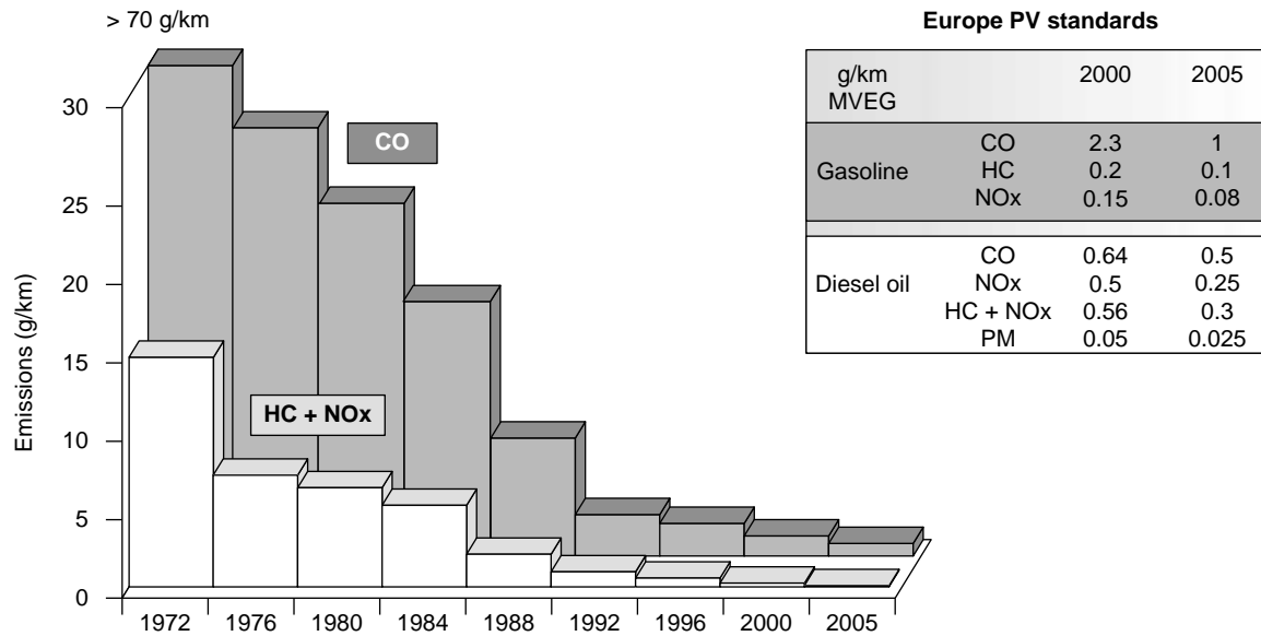
Figure 6 Evolution of the antipollution regulations since 1970 for the private cars.
