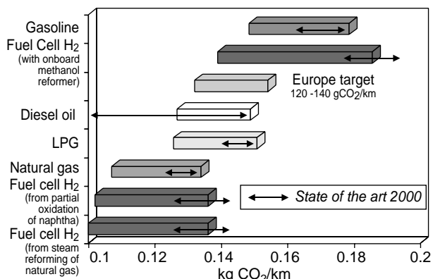
Figure 11 Well-to-wheel CO 2 emissions for various cars technologies.
