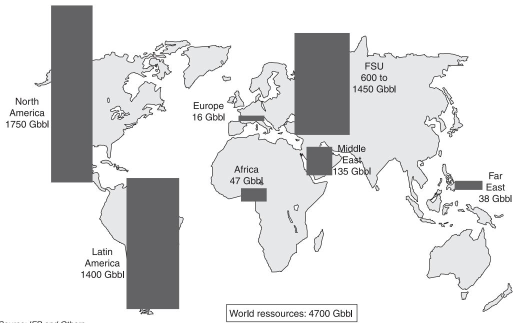
Figure 3 Geographical distribution of heavy, extra-heavy oils and bitumen resources.
