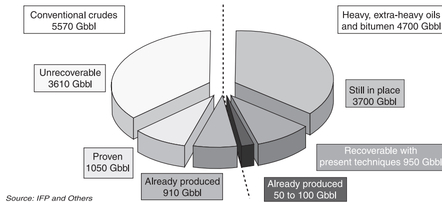
Figure 2 Distribution of identified petroleum resources in 2003.
