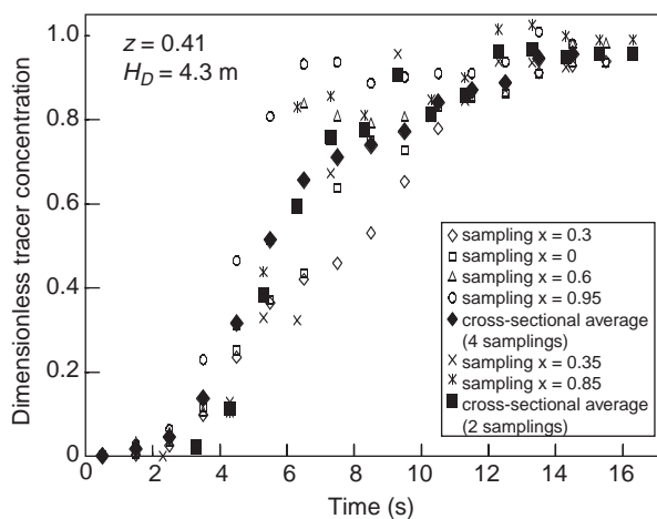
Figure 10 Cross-sectional averaged tracer concentration over two and four radial positions.
