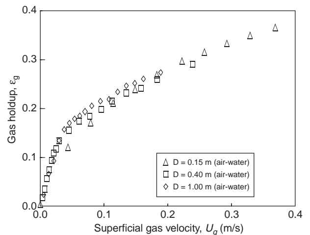
Figure 11 Global gas holdup as a function of D .
