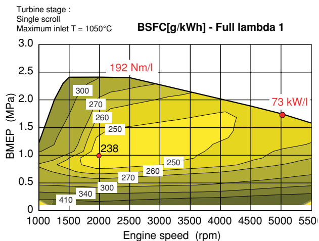
Figure 16 Mono-scroll 2.4 MPa BMEP application, full lambda-one BSFC (g/kWh) map (maximum upstream turbine temperature: 1050°C).
