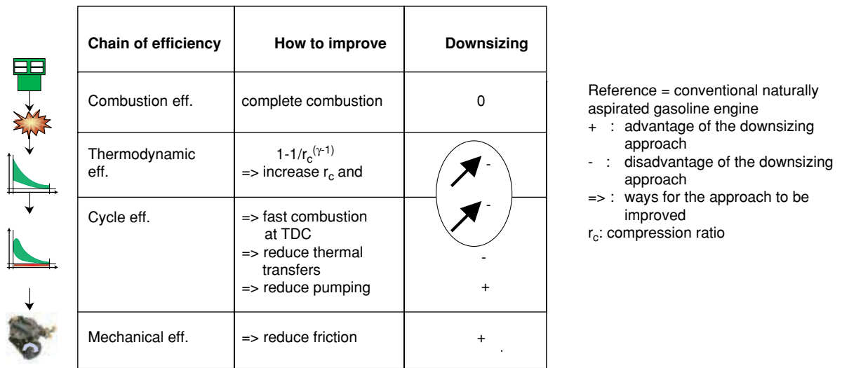
Figure 1 Improving efficiency of downsizing.
