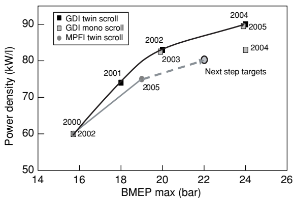
Figure 17 Progression of GDI engine specific performances and targets of PFI application.
