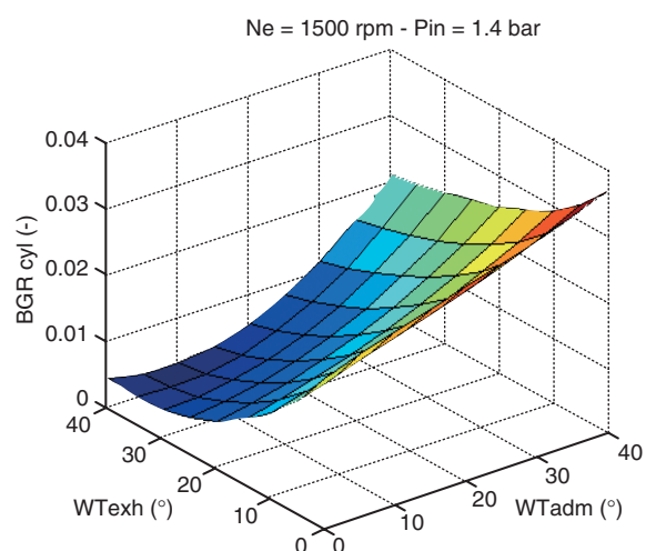
Figure 28 In-cylinder burnt gas mass in turbocharged mode for various valve timings.
