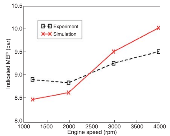
Figure 12 IMEP model/bench comparison vs engine speed.
