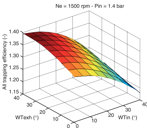
Figure 27 In-cylinder air mass observer in turbocharged mode for various valve timings.
