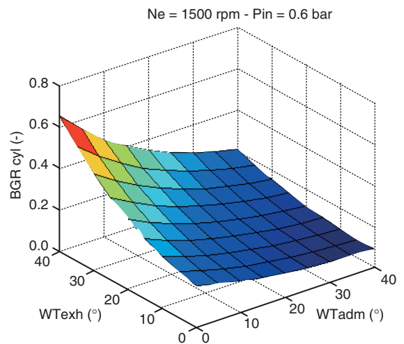
Figure 26 In-cylinder burnt gas mass observer in naturally aspirated mode for various valve timings.
