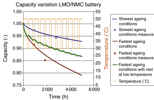
Figure 8 Simulation results representing a succession of stress and rest periods.
